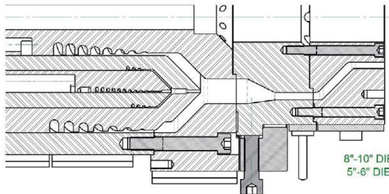
Pic. 8: Melt merging of PE/Ad/PA/Ad/PE
